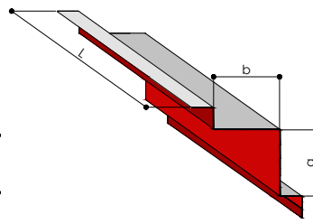
TZ-C INTERIOR ANGLE
