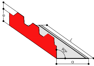
TZ-C LOWER DIE-STAMPED SLOPE FINISH (Width: 1 panel)
