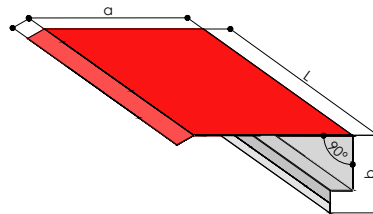
TZ-C CREST ON LATERAL SLOPE
