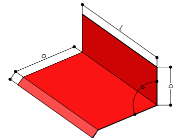
TZ-C CREST ON FACADE TO SIDE
